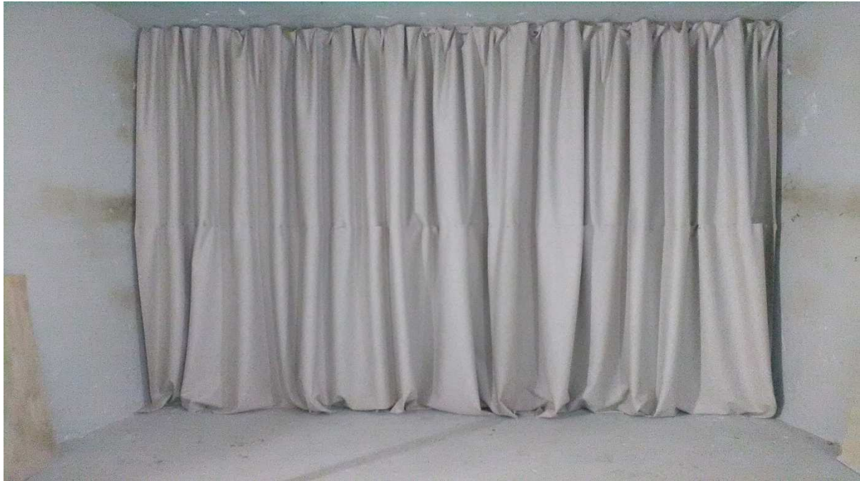
Figura 2_ Reverberation chamber with Sample Configuration 1
